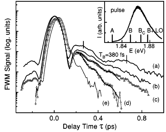
FIG. 1. Time-integrated FWM signal as a function of delay time excited by 70 fs pulses of polarization \vec{E} \parallel \vec{c} and detected at the energy of the B exciton E_B = 1.852 eV. The excitation densities are (a) 4 \times 10^{15} \text{ cm}^{-3} , (b) 3 \times 10^{16} \text{ cm}^{-3} , (c) 1 \times 10^{17} \text{ cm}^{-3} , (d) 3.7 \times 10^{17} \text{ cm}^{-3} , (e) 1.8 \times 10^{18} \text{ cm}^{-3} . Curves (c) and (d) are fitted by an oscillation period of 143 fs. The inset shows the spectrum of the exciting laser pulse and the energy positions of the A exciton (A), the B exciton (B), the B-continuum edge ( B_C ), and the B-exciton energy +\hbar\omega_{\text{LO}} ( B + \text{LO} ).
