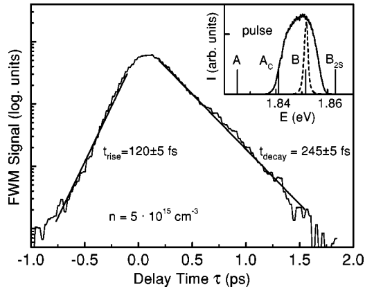
FIG. 4. Time-integrated FWM signal as a function of delay time after excitation by a pulse-shaped 210 fs pulse at E = 1.85 eV in the Markov limit (see text). The inset shows the spectrum of the exciting laser pulse (solid line) and the energy positions of the A exciton ( A ), the A -continuum edge ( A_C ), the B exciton ( B ) (dashed line, spectrum), and the energy of the B_{n=2} exciton ( B_{2S} ).
