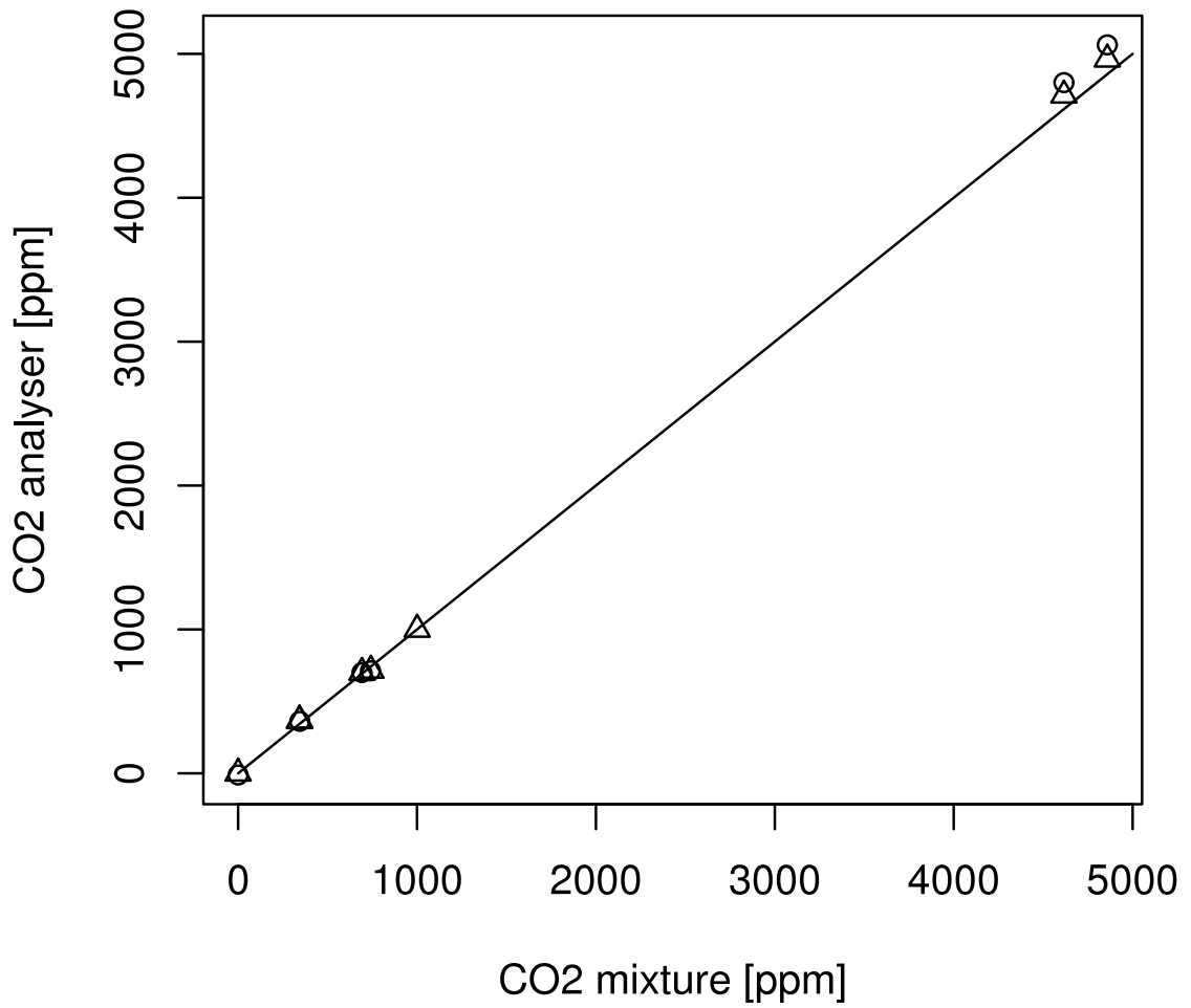
Figure C.4.: Linearity of CO 2 -analyser in carrier gases N 2 (△) and CO (○). The analyzer had been calibrated with test gas with 1001 ppm CO 2 and 1001 ppm CO in N 2 .
