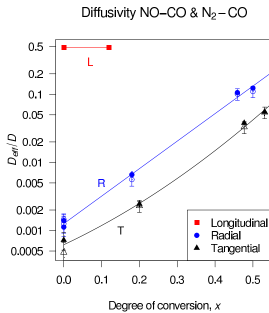
(a) Diffusion results with gas pairs NO-CO and N 2 -CO. □ ○ △: NO; ■ ● ▲: CO.
