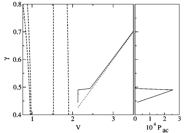
FIG. 10. I - V characteristics and the P_{ac} dependence on the dc bias current for \alpha=0.1 , \beta_L=3.0 , \eta=0.5 .
