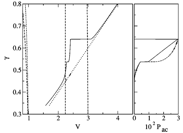
FIG. 9. I - V characteristics and the P_{ac} dependence on the dc bias current for \alpha=0.1 , \beta_L=1.0 , \eta=0.5 .
