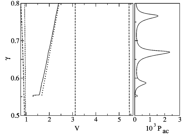
FIG. 5. I - V characteristics and the P_{ac} dependence on the dc bias current for \alpha=0.1 , \beta_L=0.2 , \eta=1.15 .
