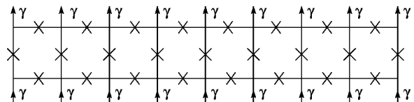
FIG. 1. Josephson junction ladder. Crosses mark the individual junctions. Arrows indicate the direction of external current flow (dc bias \gamma ).
