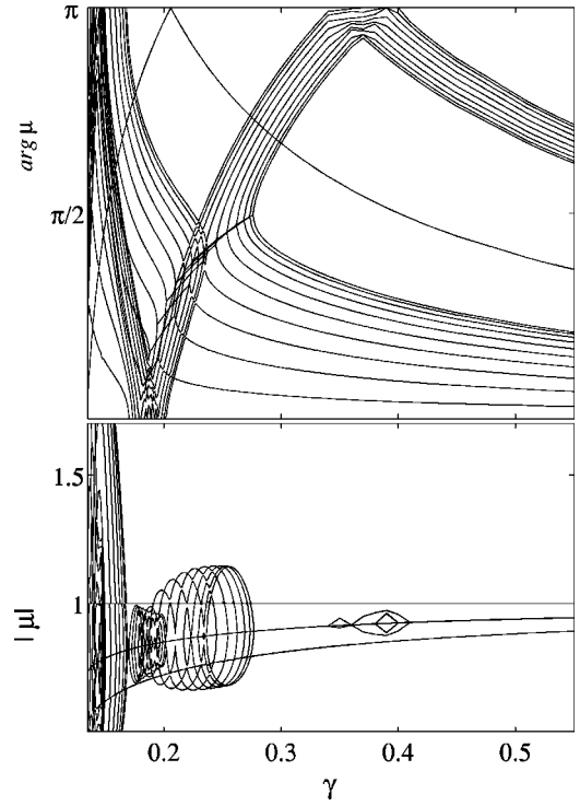
FIG. 13. Arguments and absolute values of Floquet multipliers versus \gamma for the HWS in Fig. 11.
