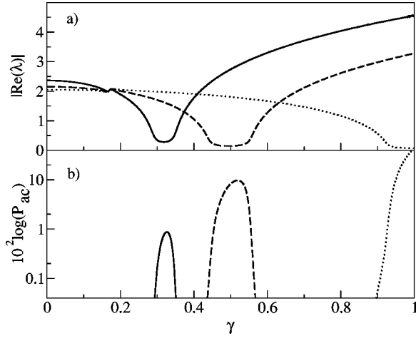
FIG. 4. (a) \text{Re}(\lambda) and (b) P_{ac} versus \gamma for different values of the inductance of the cell: \beta_L=3 , solid line; \beta_L=1 , dashed line; \beta_L=0.2 , dotted line. All of these curves are for a left-right symmetry breather with k=1 .
