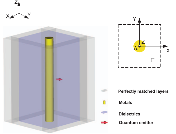
FIG. 4. (Color) A single quantum emitter coupled to a metallic nanowire. The gray transparent region represents the perfectly matched layers, the mode matching boundary condition is applied on the top and the bottom of the structure. The quantum emitter is implemented by an electric line current.
