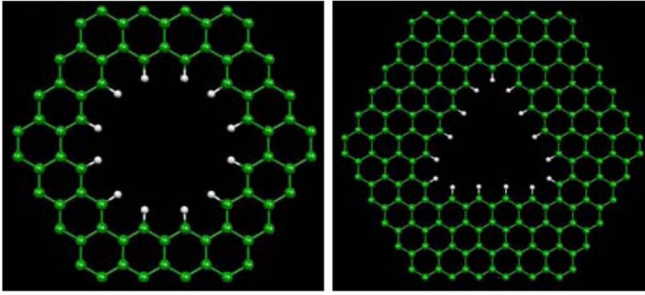
FIG. 1. (Color online) The unit cell of the \{4,2\}_O (left) and \{6,5\}_\Delta (right) system. The hexagonally shaped unit cells are repeated in plane to form a honeycomb lattice of antidots. The carbon atoms (green/gray) are hydrogen terminated (white) along the hole edges.
