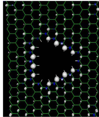
FIG. 5. (Color online) The difference in majority spin and minority spin densities for the \{6,5\}_{\Delta} structure. Blue/dark gray (white) indicates surplus of majority(minority) spin.
