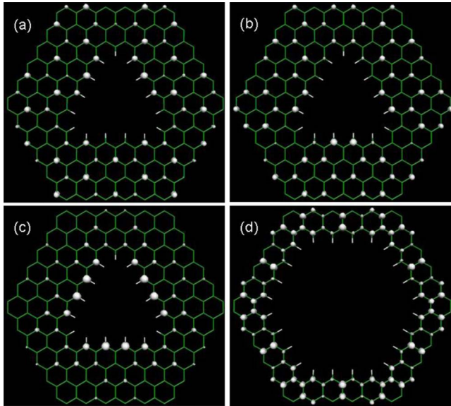
FIG. 4. (Color online) Amplitudes of certain important states. (a,b): degenerate midgap states, (c): nondegenerate midgap state of \{6,5\}_{\Delta} , (d): highest filled bands of \{6,3,6\}_{\circ} . All states are calculated at the \Gamma point.
