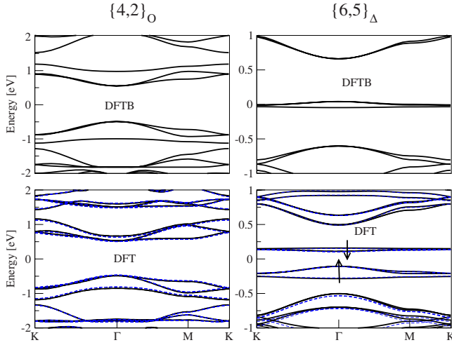
FIG. 3. (Color online) Band structures for the \{4,2\}_O (left column) and \{6,5\}_\Delta (right column) systems using DFTB (upper panels) and DFT (lower panels). The dotted blue/dark gray curves in the lower panels are DFT results using structures relaxed with DFTB. The arrow pointing up (down) indicates that bands are filled with majority (minority) electrons only.
