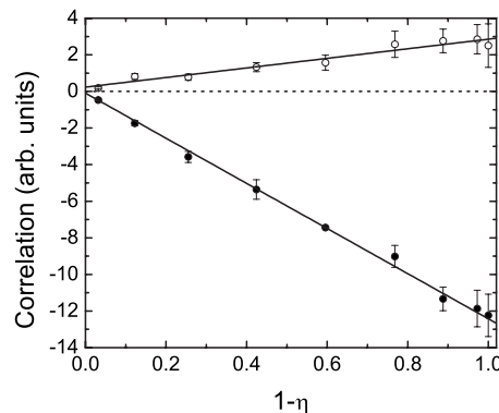
FIG. 5. The covariance at the maximally squeezed (open circles) and the maximally antisqueezed quadrature (filled circles) versus the transmittance of the LO ( 1 - \eta ).
