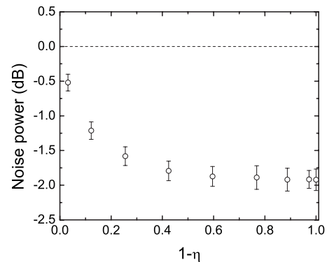
FIG. 8. Measurement along the squeezed quadrature in the OPA-based squeezing setup using homodyne detection. The plot shows how the degree of squeezing depends on the transmission of the LO ( 1-\eta ).
