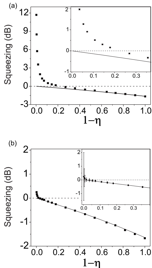
FIG. 9. Experimental dependence of the amount of squeezing on the transmission ( 1 - \eta ) (a) for homodyne detection and (b) for the covariance method. The solid lines represent the theoretical prediction without accounting for the EN. The horizontal dashed line at zero marks the border between squeezing and classical excess noises.
