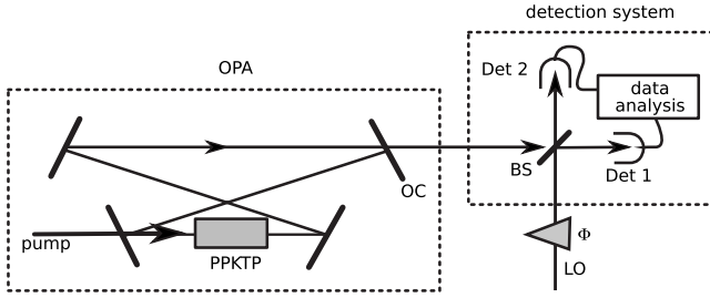
FIG. 3. The scheme of the OPA based setup. A frequency-doubled Nd:YAG laser (fundamental wavelength of 1064 nm) is used to pump the bowlike-shaped OPA with a 10-mm-long periodically poled Potassium Titanium Oxide Phosphate (PPKTP) crystal. The squeezed vacuum field, generated by the OPA, is mixed with the fundamental wave of the pump laser on a 50:50 BS, used as a LO, and further detected by two analog photodetectors (Det 1 and Det 2). The relative phase between the squeezed vacuum field and the LO is controlled by a mirror on a piezostage (not shown). The photocurrents of two detectors are further analyzed by the high-speed digitizer.
