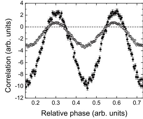
FIG. 4. The covariance versus the phase of the LO at two different powers of the LO (open and filled circles) for the OPA-based squeezing setup. Positive covariance values correspond to the measurement of the squeezed quadrature, while the negative covariance values correspond to the measurement of the antisqueezed quadrature.
