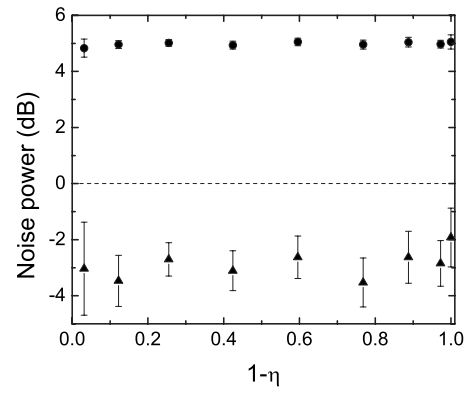
FIG. 7. The degree of squeezing (triangles) and antisqueezing (circles) revealed from the correlation analysis versus the transmittance of the LO ( 1-\eta ) in the OPA-based squeezing setup. The relatively large error bars are mostly due to statistical fluctuations.
