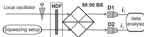
FIG. 1. Schematic of the setup. The beam from the squeezing setup [optical parametric amplifier (OPA) or Kerr-based squeezing setup (see text)] is interfering with the LO on a 50:50 BS, with a relative phase of \phi . D1 and D2 are the analog photodetectors. The photocurrents of the detectors i_1 and i_2 are analyzed by the acquisition system.
