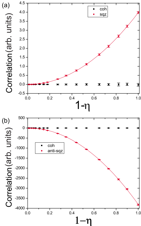
FIG. 6. (Color online) Effect of the transmittance of the LO ( 1-\eta ) on the covariance at (a) the maximally squeezed and (b) the maximally antisqueezed quadrature. In both plots we compare the covariance of a squeezed beam (red) to a calibration measurement using a coherent beam (black).
