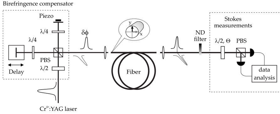
FIG. 2. The scheme of the polarization squeezing setup. The beam from the \text{Cr}^{4+} :yttrium aluminum garnet (YAG) laser is split on the polarization beam splitter (PBS) after polarization rotation, performed by a half-wave plate (HWP). The birefringence compensator is used to provide a temporal overlap between two orthogonally polarized pulses after propagation through a single-mode polarization maintaining fiber. The interference between the pulses is observed by placing a HWP and a PBS in front of two analog photodetectors. The photocurrents of two detectors are further analyzed by the high-speed digitizer.
