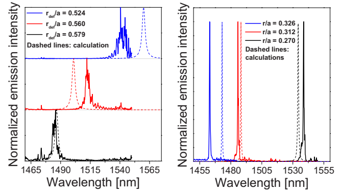
FIG. 2. (Color online) (left) Cavity mode of H1-r designs with fixed r/a=0.27 and various defect radii r_{\text{def}}/a compared with calculations depicted as dashed lines. (right) Cavity mode of L3 designs with various hole radii r/a compared with calculations.
