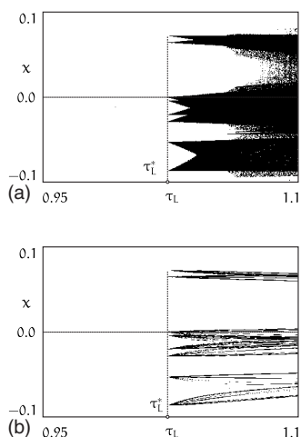
FIG. 5. Birth of an eight-band strange attractor through a smooth period doubling coinciding with a border-collision bifurcation. (a) One-parameter bifurcation diagram for the section along the direction A in Fig. 4, \tau_R = -1.0 . (b) Birth of a family of unstable cycles with periods that are multiples of 4. The cycles arise through the border-collision bifurcation at the point \tau_L^* \approx 1.0236 . This diagram contains the unstable cycles with the periods 4, 8, 16, 24, 32, and 40.
