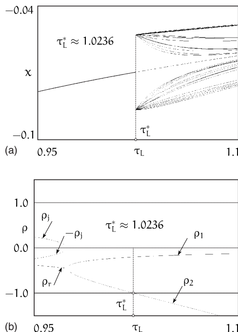
FIG. 6. (a) Magnified part of the bifurcation diagram presented in Fig. 5(b) showing the evolution of one branch. (b) Multiplier diagram illustrating the smooth period doubling of the period-4 cycle. At the point \tau_L^* \approx 1.0236 the largest multiplier (in absolute value) of the period-4 cycle crosses through -1 . The loss of stability of the period-4 cycle is not accompanied by the appearance of a stable period-8 cycle. Rather a whole family of unstable cycles arise through the border-collision bifurcation at \tau_L^* [see Figs. 5(b) and 6(a)].
