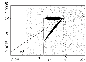
FIG. 12. Hard transition to chaos through period-doubling and homoclinic bifurcations, \tau_R = -0.82 . \tau_L^H is the point of the second homoclinic contact, and \tau_L^* is the point of the period-doubling bifurcation.
