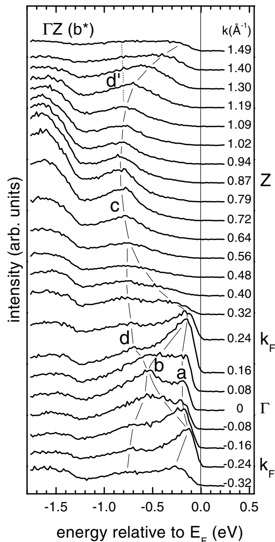
FIG. 2. Angle-resolved photoemission spectra measured for wave vectors k along the \Gamma Z direction ( h\nu = 25 eV, T = 61 K). The thin lines indicate the dispersion of the spectral features.
