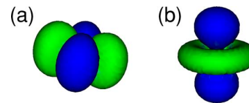
FIG. 7. (Color online) Two d -like WFs for Cu(fcc). The orbitals are centered at the atoms (not shown).
