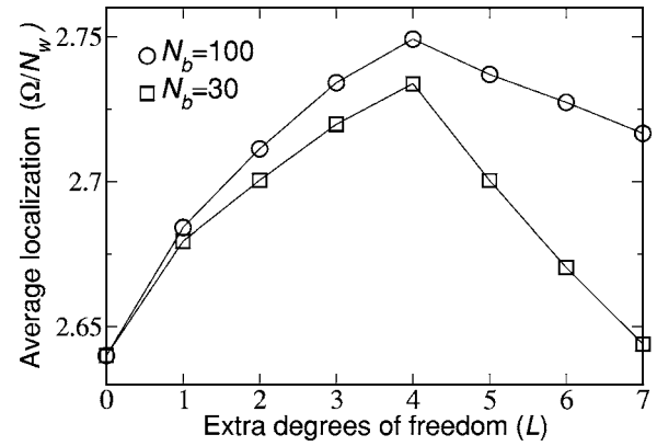
FIG. 4. Average spread of the WFs of the \text{Si}_5 cluster for different values of N_b and L .
