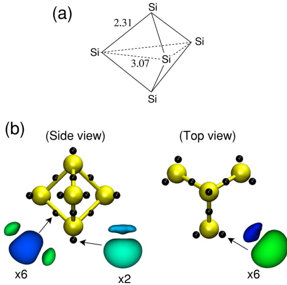
FIG. 3. (Color online) (a) Geometry of the \text{Si}_5 cluster. (b) Contour plots of the WFs corresponding to L=4 . The position of the WF centers are indicated by black spheres.
