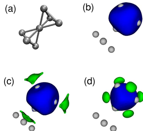
FIG. 8. (Color online) (a) Two tetrahedral interstitial sites in the fcc crystal. (b)–(d) Contour plots of the s -like WF obtained for Cu (fcc). The WFs in (b) and (c) have been generated with N_w=6 , E_0=0.0 eV and N_w=6 , E_0=3.0 eV, respectively. Both WFs are located in one of the interstitial sites. The WF in (d) corresponds to N_w=7 and E_0=0.0 eV. In this case there is an equivalent WF located in the other interstitial site. The same contour value has been used for all plots.
