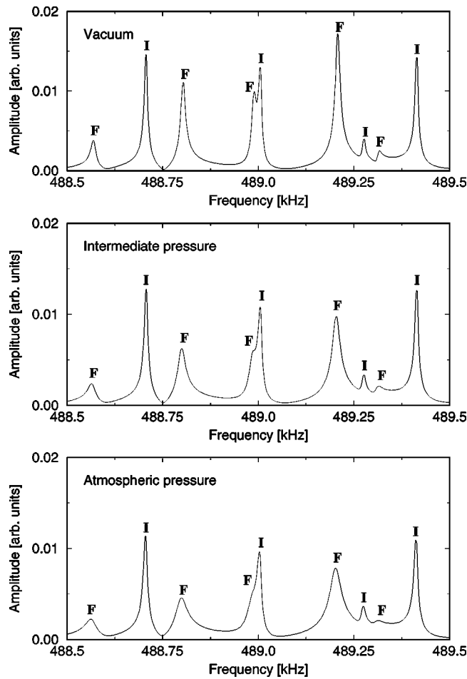
FIG. 6. A segment of the resonance spectrum for the 2-mm-thick three-leaf clover at three different pressures: vacuum, 0.5 atm, and 1 atm. Most resonances are easily recognized to be either in-plane (I) or flexural (F).
