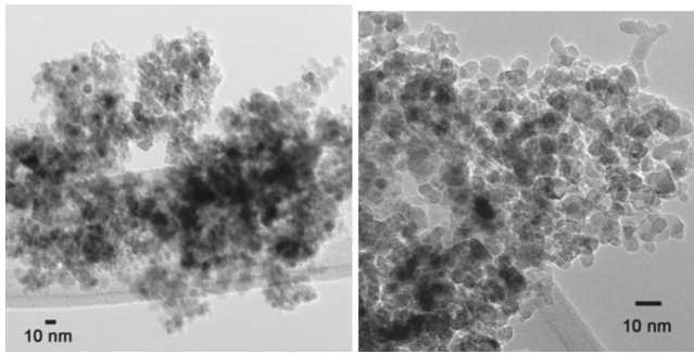
FIG. 1. Transmission electron microscopy of the 260-ARG (left) and 260-ARG-AIR (right) aerogels.
