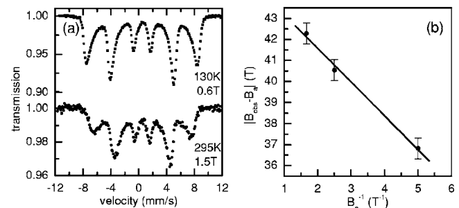
FIG. 3. (a) Mössbauer spectra of the 260-ARG aerogel at the indicated temperatures and applied fields. (b) Field dependence of the induced hyperfine field at 295 K used for the size estimation in sample 260-ARG-AIR.
