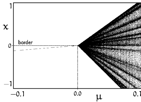
FIG. 1. Bifurcation diagram for the normal form map as the parameter \mu varies from -0.1 to 0.1 . The diagram shows a direct transition from a period-1 orbit to a quasiperiodic orbit. The other parameters are \tau_L = 0.6765 , \tau_R = 1.5 , \delta_L = 0.5 , and \delta_R = 1.6 .
