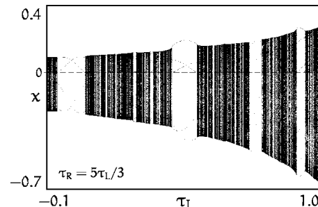
FIG. 3. Bifurcation diagram calculated for the section \{(\tau_L, \tau_R) : -0.1 \leq \tau_L \leq 1.0; \tau_R = 5\tau_L/3\} situated along the main diagonal of Fig. 2. The diagram shows repeated transitions between mode locking and quasiperiodicity.
