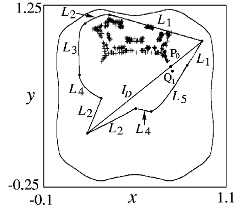
FIG. 8. Synchronous attractor I_D and its basin boundary (outer closed curve) after the transcritical riddling bifurcation. By black crosses, a number of periodic orbits belonging to the chaotic saddle \tilde{A}_{up} are indicated. Also shown is the boundary of the semi-invariant absorbing area \mathcal{A} that is created by arcs L_k, k = 1, \dots, 5 that are the images of critical lines L_0 from (5). Parameters are a = 3.8, p = 0.27 , and \varepsilon = 1.58 .
