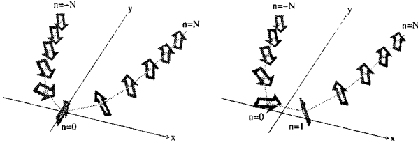
FIG. 1. DNA chain embedded on a parabola in the xy plane. Sites (x_n, y_n) with y_n = (\kappa/2)(x_n - \gamma)^2 , indicated by light gray dots. Base pair dipoles, orthogonal to the parabola, shown as dark gray arrows. Curvature \kappa=2 and twist \tau=1 . The z -axis (not shown) forms a right-handed system with x and y axes. Left, the on-site case, \gamma=0 . Right, the intersite case, \gamma=1/2 .
