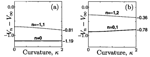
FIG. 8. Effective potential V_n - V_\infty for constant twist. (a) On-site case, \tau = 6 . (b) Intersite case, \tau = 2 .
