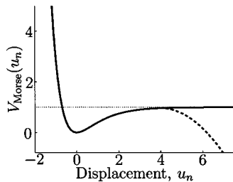
FIG. 2. The Morse potential V_{\text{Morse}}(u_n) = (e^{-u_n} - 1)^2 (solid curve). Effective potential, Eq. (9), in the analytical approximation (dashed curve).
