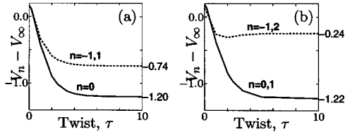
FIG. 7. Effective potential V_n - V_\infty for constant curvature \kappa = 1.0 . (a) On-site case. (b) Intersite case.
