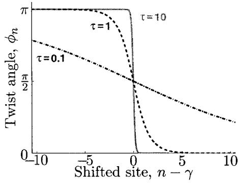
FIG. 3. (Color online) The twist angle, \phi_n , for various values of the twist, \tau , around the chain center. On-site case, \gamma=0 ; intersite case, \gamma=1/2 .
