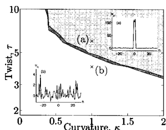
FIG. 5. Region of bubble generation in the on-site case. Light gray region, bubble generation. Dark gray region, transition region indicating the uncertainty of the simulations. White region, no bubble generation. Insets show the displacement, u_n , versus site, n , at the points (a) and (b) at simulation times (a) t=51 and (b) t=100 for the same initial condition.
