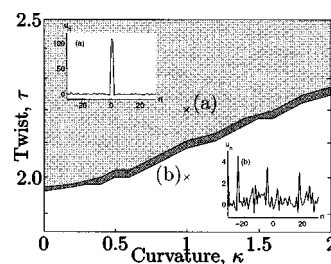
FIG. 6. Region of bubble generation in the intersite case. Light gray region, bubble generation. Dark gray region, transition region indicating the uncertainty of the simulations. White region, no bubble generation. Insets show the displacement, u_n , versus site, n , at the points (a) and (b) at simulation time (a) t=45 and (b) t=100 for the same initial condition.
