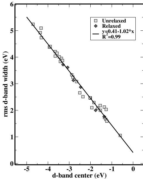
FIG. 1. Correlation between the root mean squared (rms) d -band width and d -band center for bimetallic surfaces.
