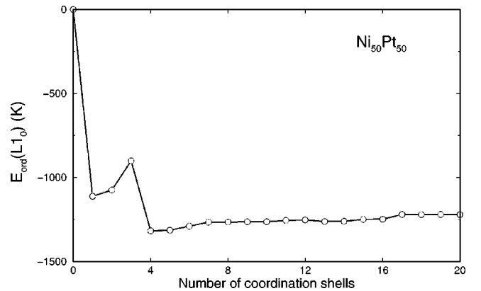
FIG. 1. The ordering energy E_{ord} (in K) of the L1_0 structure as a function of the number of coordination shells included in the calculation.
