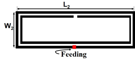
Fig. 8. Self Resonant Split Ring Antenna.
