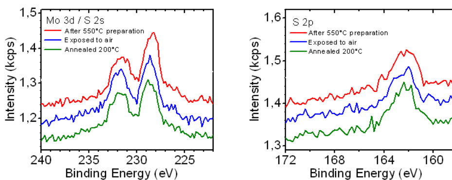
Figure 4.12: XPS spectra of the Mo 3d and S 2s binding energy region on the left and the S 2p region on the right. Red: As prepared sintered \text{MoS}_2 on \text{Au}(111) sample. Blue: The same sample after air exposure. Green: The same sample after annealing to 200^\circ\text{C} .
