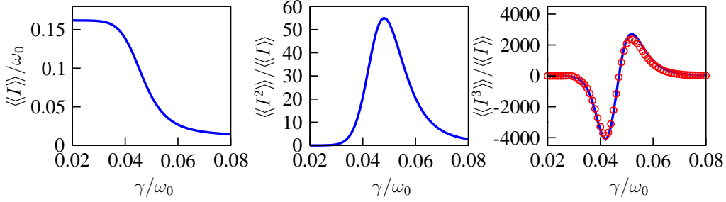
Figure 4.3: First three current cumulants of the quantum shuttle as function of the damping \gamma . Full lines show numerical results, while circles correspond to Eq. (4.53). Parameters are \Gamma_L = \Gamma_R = 0.01\omega_0 , \lambda = 1.5x_0 , d = eE/m\omega_0^2 = 0.5x_0 , x_0 = \sqrt{\hbar/m\omega_0} . Figure from Paper F .
