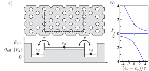
FIG. 5: (a) The structure considered for resonant coupling of distant defect states; two defects separated by a central line of N = 3 antidots, with a central back gate V_g controlling the potential square well in the region marked with dashed lines. A simple three-level model of the system is illustrated below. (b) The eigenvalue spectrum of the three-level model. The dashed line marks the point of resonance.
