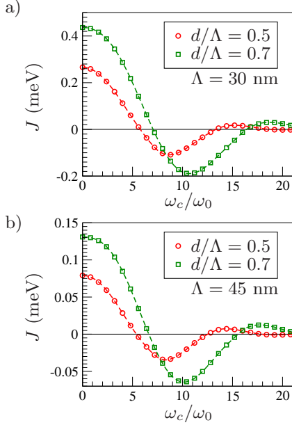
FIG. 9: (Color online) Exchange coupling J for a double defect structure as a function of \omega_c/\omega_0 , where \omega_c = eB/m^*c and \omega_0 = \hbar/(2m^*\Lambda^2) . Results are shown for a relative split gate constriction width w/\Lambda = 2 , and two different values of the relative antidot diameter d/\Lambda . The lattice constant is (a) \Lambda = 30 nm and (b) \Lambda = 45 nm.
