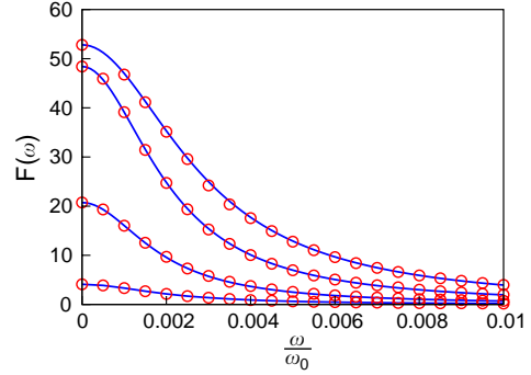
Fig. 3. The ratio between the current noise and the current F(\omega) = S_{II}(\omega)/\langle \hat{I} \rangle for low frequencies ( \omega \ll \omega_0 ). The parameters are \gamma = 0.035\omega_0 (lowest curve), 0.04\omega_0, 0.045\omega_0, 0.05\omega_0 (top-most curve), \Gamma_L = \Gamma_R = 0.01\omega_0 , \lambda = 1.5x_0 , d \equiv eE/m\omega_0^2 = 0.5x_0 , where x_0 = \sqrt{\hbar/m\omega_0} . The circles indicate numerical results, while the full lines indicate the analytic results for the current noise spectrum of a bistable system. It should be noted that in order to obtain the agreement between the numerical and analytic results it is necessary to assume that the shuttling current for the given values of \gamma is not fully saturated to the value I_{\text{shut}} = 1.03\omega_0/2\pi . Corresponding to the different values of \gamma we have used I_{\text{shut}} = 1.01\omega_0/2\pi (for \gamma = 0.03\omega_0 ), 1.00\omega_0/2\pi , 0.98\omega_0/2\pi , 0.94\omega_0/2\pi (for \gamma = 0.05\omega_0 ), respectively.
