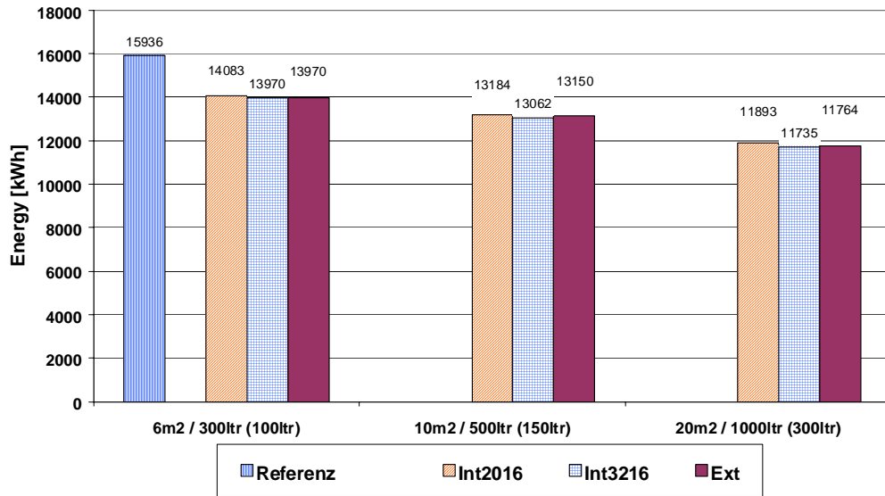
Fig. 4–9 Yearly auxiliary demand of the reference system and the three system sizes with the three system concepts, respectively.
