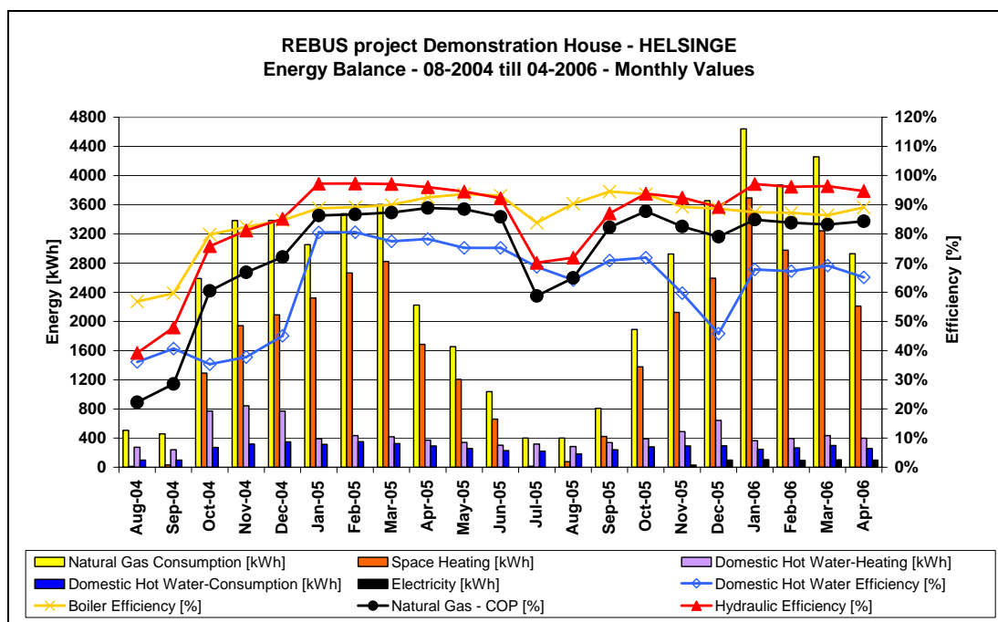
Fig. 6–15 Energy balance for the old heating system in the demonstration house.
