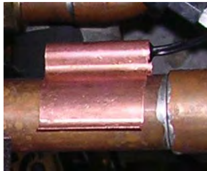
Fig. 5–8 Advanced standard sensor based on a NTC element in a copper cylinder with a copper clamp to be clipped on a pipe.
