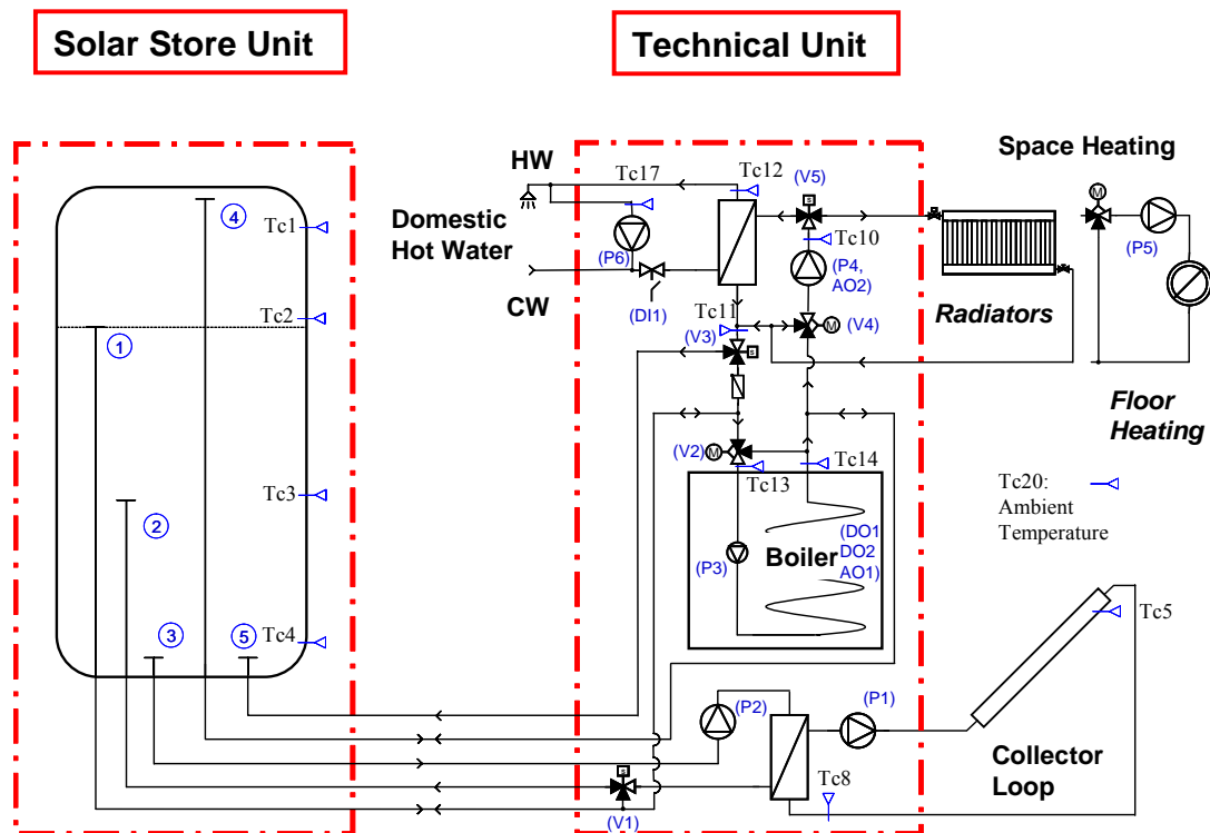
Fig. 5–1 Principle hydraulic scheme of the solar combisystem concept
