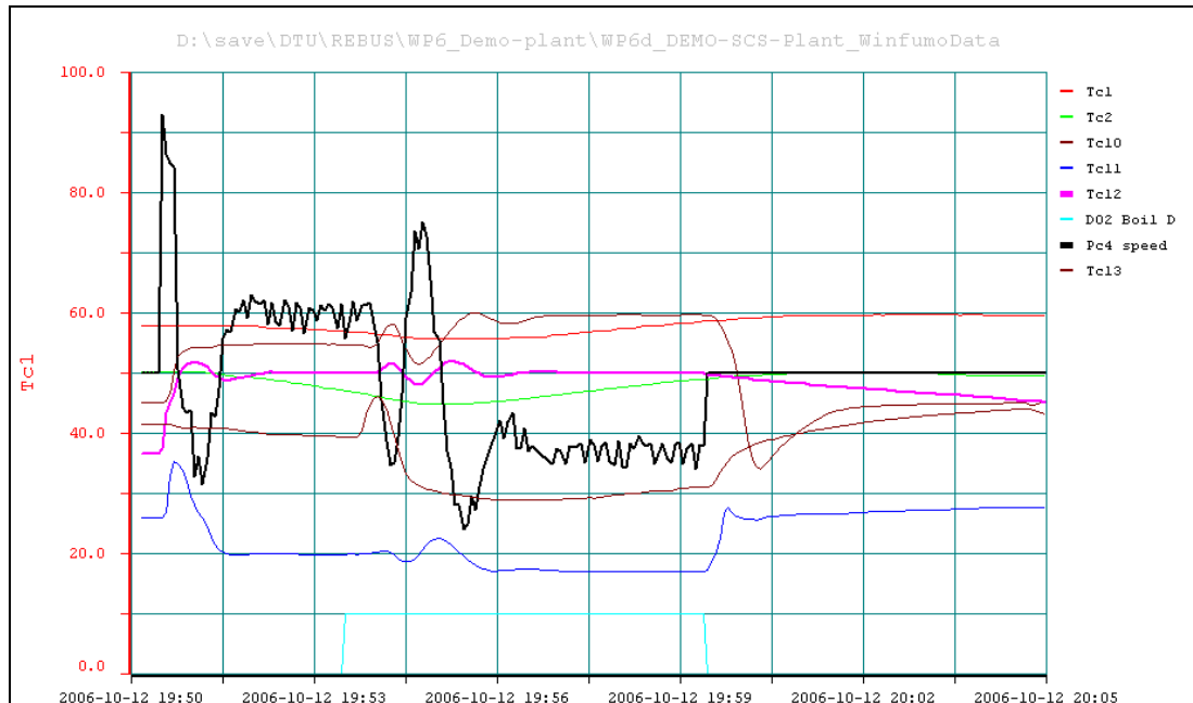
Fig. 5–16 Hot water preparation with boiler starting during tapping with the final control algorithm for the 3-way valve (Vc2) (Tc1-Tc20 in °C / Pc4_speed in % / DO2_Boil_D is an on/off signal).
