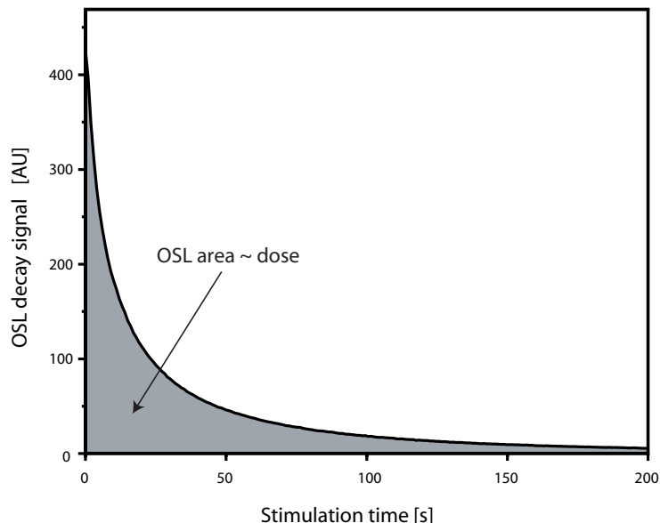
Figure 1.1: A cw-OSL decay curve from \text{Al}_2\text{O}_3\text{:C} crystal after a 2.7 Gy irradiation with a ^{137}\text{Cs} \gamma -source. The area under the OSL curve is ideally proportional to the dose.
