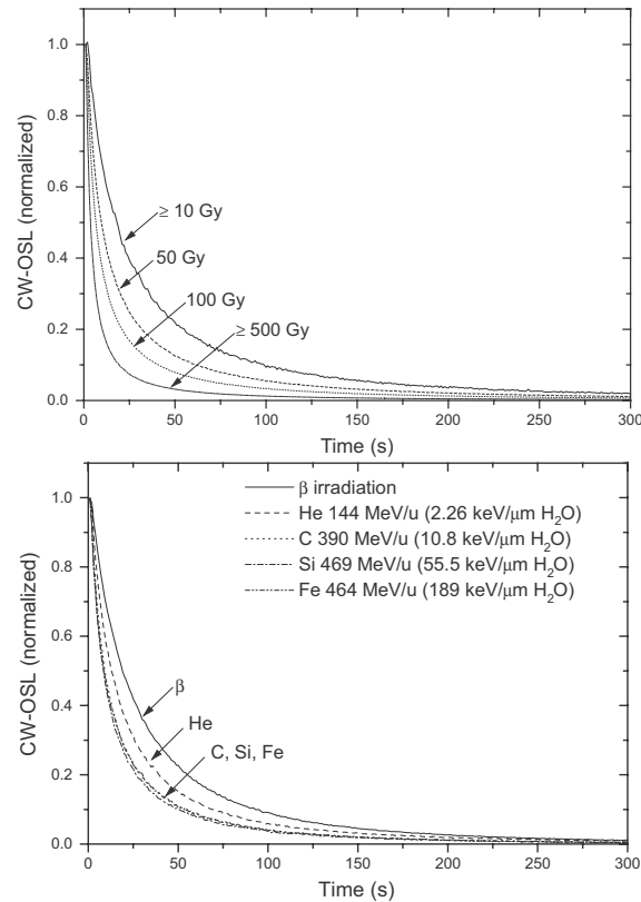
Figure 5.3: Normalized cw-OSL decay curves from Luxel™ \text{Al}_2\text{O}_3:\text{C} dosimeters given by Yukihara et al. [95]. Upper: Dosimeters exposed to \beta -irradiation with a ^{90}\text{Sr} source. Numbers indicate the dose given in Gy. Lower: Dosimeters given a dose of 0.1 Gy with different ionization densities (LET) as indicated in the figure.
