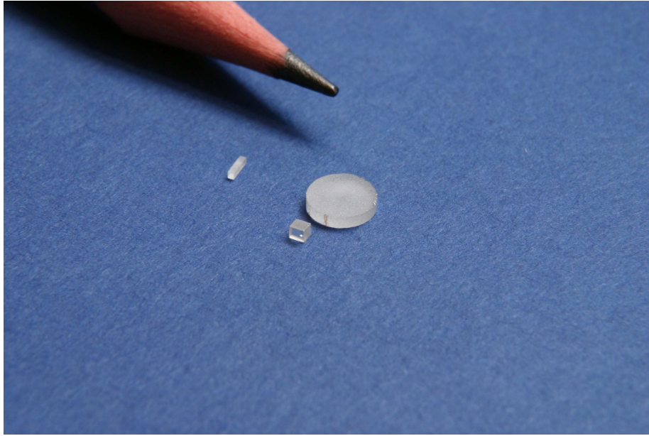
Figure 3.5: The two types of \text{Al}_2\text{O}_3:\text{C} crystals named TLD-500 (right) and CZ#60 (left). The TLD-500 crystal is cut from a standard pellet as the one shown in the figure.
