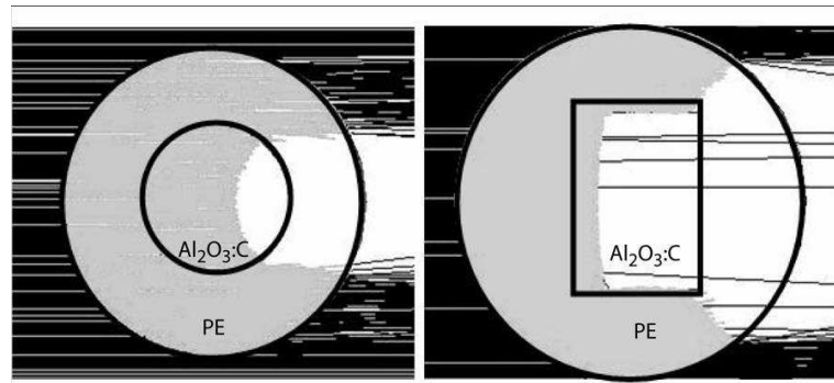
Figure 5.13: A cross-sectional view of a GEANT4 simulation of 10 MeV protons in probe A and B. The protons enters the geometries of probe A (left) and probe B (right) from the left. In the simulation, the \text{Al}_2\text{O}_3:\text{C} crystals are covered with polyethylene (PE). Black areas: protons, dark gray areas: energy deposition, light gray areas: no energy deposition. The simulation was kindly provided by Gabriel Sawakuchi, Oklahoma State University (USA), 2006.
