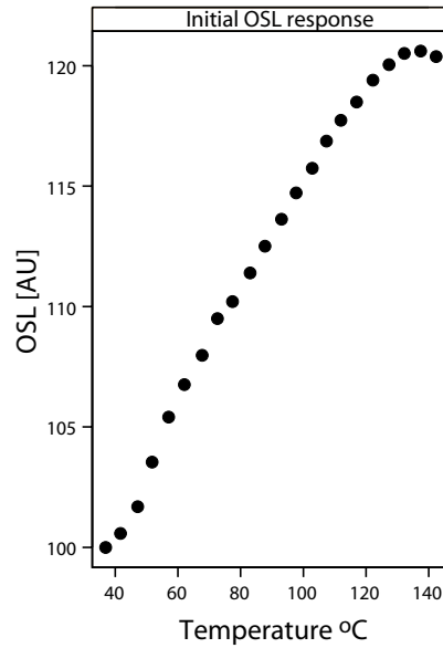
Figure 4.1: The initial OSL signal versus temperature as published by Markey et al. [58]. The sample was irradiated with 1.5 Gy at room temperature whereafter it was heated at a linear rate of 2 °C per sec from room temperature to 550 °C. During the heating, the sample was exposed to periodic green light stimulations of 0.1 s duration. In this way, the initial OSL signal is monitored with increasing stimulation temperature. The decrease in signal starting around 130 °C is believed to be partially due to the emptying of the main dosimetry trap and partially due to thermal quenching.
