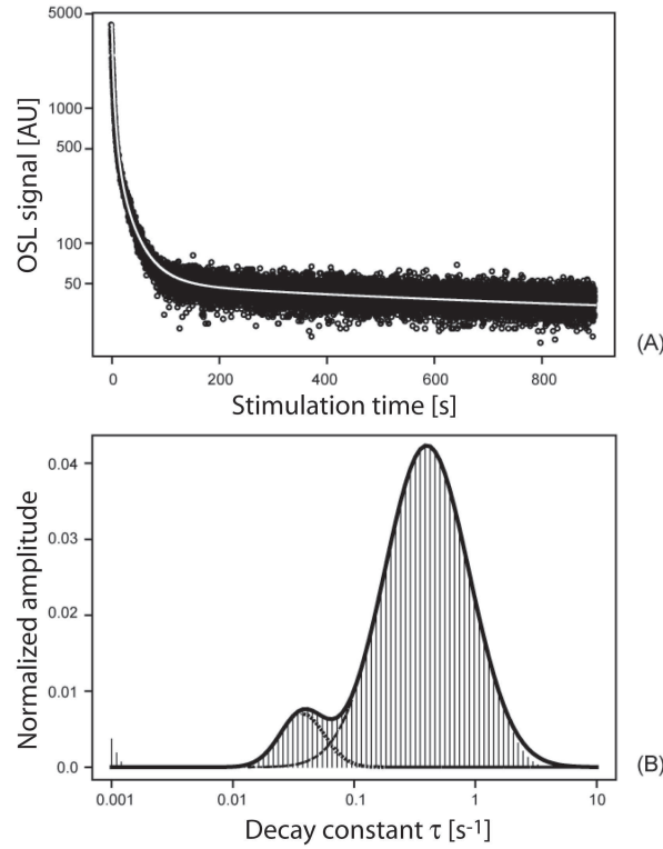
Figure 2.6: A: An OSL decay curve (black circles) and a fitted curve (white line) from Al 2 O 3 :C using Tikhonov regularization. B: Corresponding spectrum of optical threshold values covering 4 decades. Small decay constants correspond to large optical threshold energies and vice versa. The lines indicate two individual Gaussian curves and their sum.
