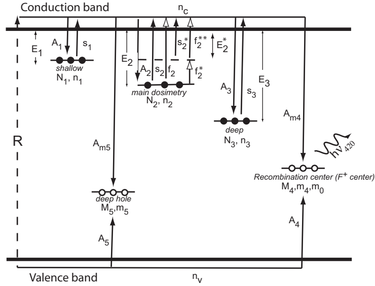
Figure 2.5: Energy band model describing charge transitions through the delocalized bands in Al 2 O 3 :C. Parameters are placed next to the process they describe. Subscripts: 1=shallow traps, 2=main dosimetry trap, 3=deep trap, 4=radiative hole trap, 5=non-radiative hole trap, and asterix=thermal excitation parameters. Optical transitions are indicated by open upwards arrows, whereas passive trapping and thermal assistance is indicated with closed arrows. Filled circles=electrons and open circles=holes. See also text for details.
