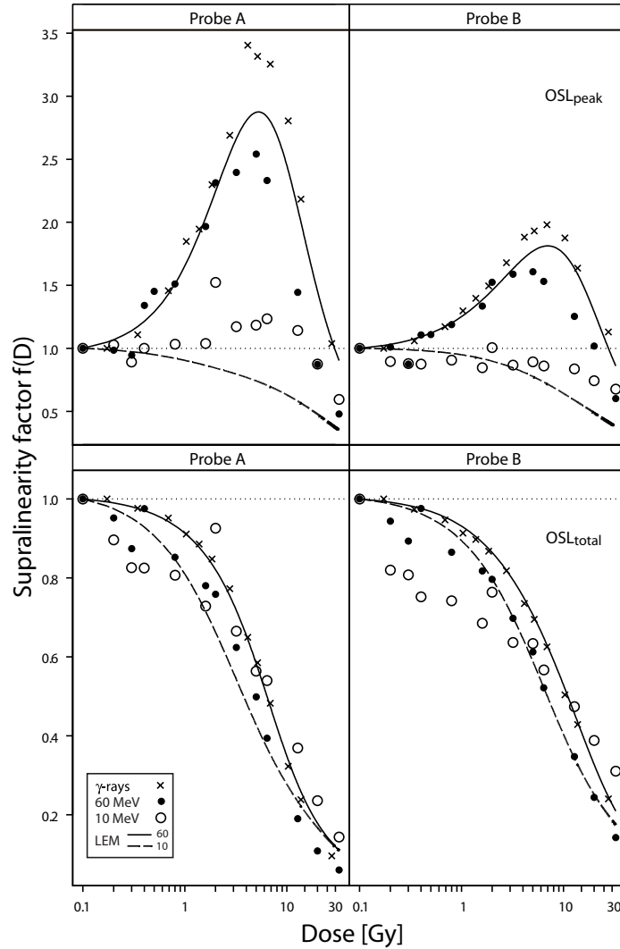
Figure 5.11: The supralinearity factor f(D) defined in eq. (2.34). The model calculations are shown with full and dashed lines and made with D_{LEM} in eq. (5.1) for 10 and 60 MeV protons in \text{Al}_2\text{O}_3 . Experimental data are shown for \gamma -rays and 60 and 10 MeV protons. The upper panels show the peak OSL signal and the lower panels show the total OSL signal.
