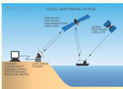
Fig. 1. Vessel Monitoring System (VMS). Taken from the Australian Fisheries Management website.
