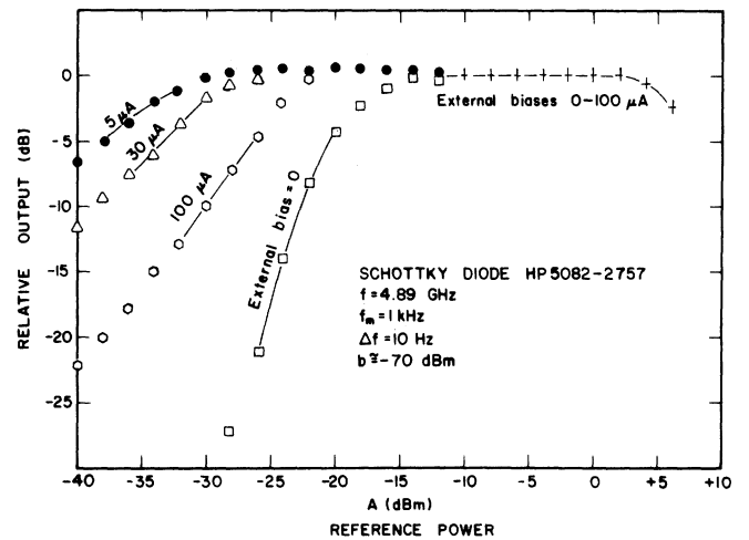
Fig. 7. Relative output of Schottky diode versus A with external bias as parameter and fixed information signal input ( -70 \text{ dBm} ).
