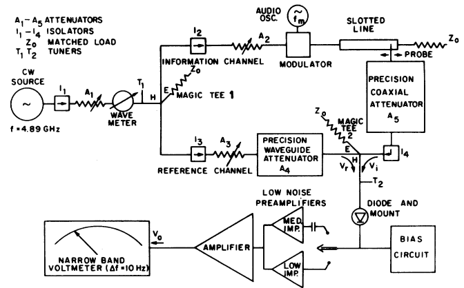
Fig. 2. Microwave homodyne system for testing detection characteristics of various diode types.
