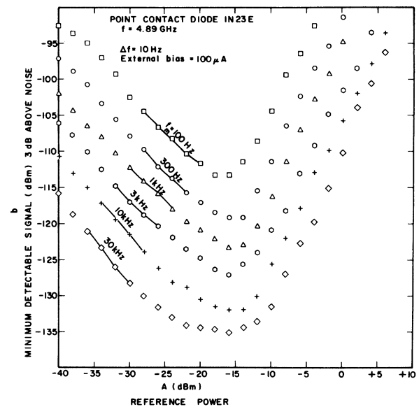
Fig. 5. Minimum detectable signal for point contact diode versus A with fixed external bias and modulation frequency f_m as parameter.
