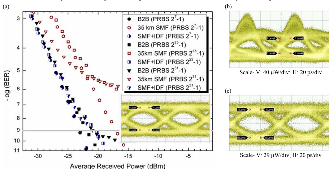
Figure 2: (a) Receiver BER as a function of receiver power for different PRBS, at points along the PON uplink: back to back (B2B), after 35 km SMF and after 50 km combined SMF+IDF. Inset shows eye diagram at VCSEL (2.4 dB extinction ratio, ER. Scale: V:20 \mu W/div, H: 20 ps/div). (b) Eye diagram after 35 km SMF (1.73 dB ER) and (c) after 50 km transmission over SMF+IDF (2.4 dB ER).
