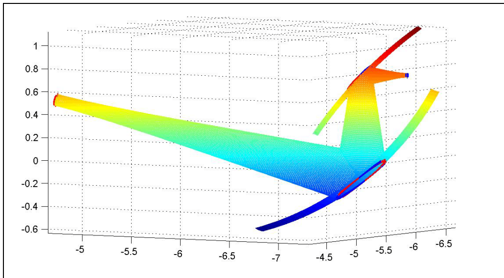
Figure 26: Modelling of the mirror shapes and the centre beam of the LFS CTS receiver
