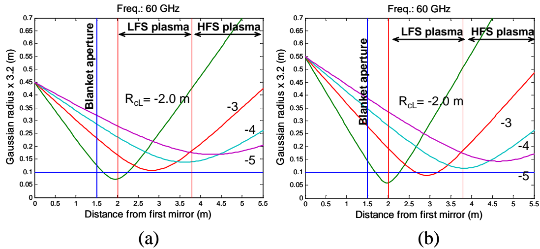
Figure 31 Beam diameters (Gaussian radius \times 3.2) as functions of distance from front-end mirror for the mirrors at 1.5 meters further inward.
