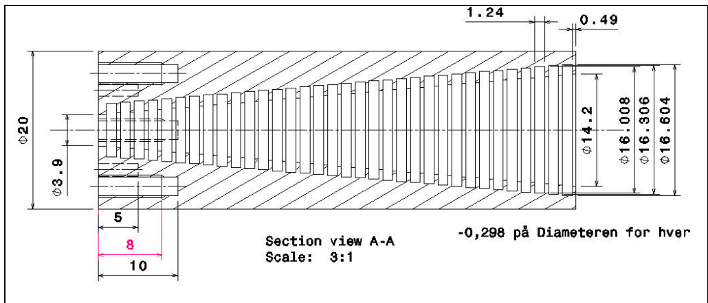
Figure 3: Design drawing of the corrugated antenna horn for 60 GHz. The overall length of the horn is 60 mm. The left side shows the interface to a circular fundamental waveguide.
