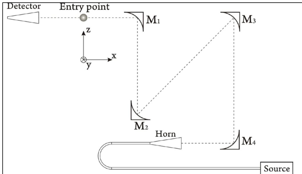
Figure 7: Schematic of receiver system and detector. The detector is movable in the y-z-direction. Mirror M1 is the plasma facing mirror.
