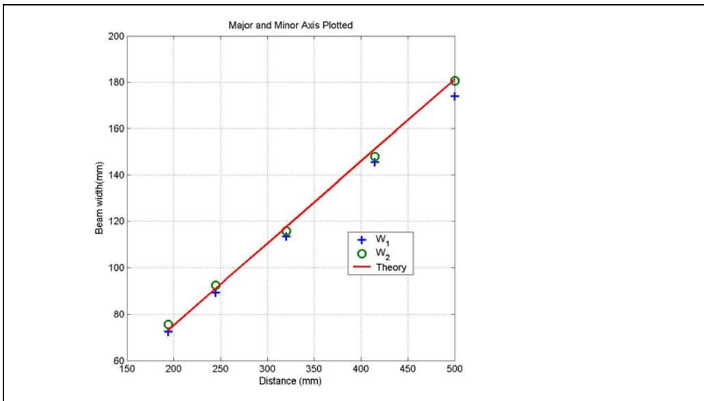
Figure 6: Envelope of the beam leaving the horn. W_1 and W_2 should be identical, as the horn has a circular symmetry. The difference is less than 3% between the measured beams in two orthogonal directions.
