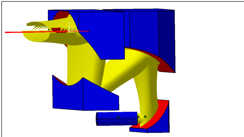
Figure 8: 3D picture from CATIA of the HFS receiver antenna.
