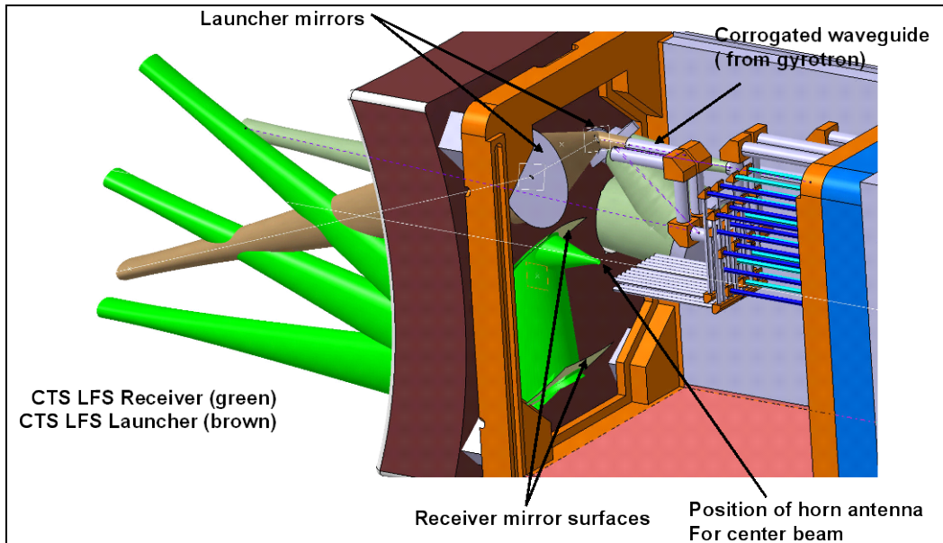
Figure 27: Equatorial port #12 on ITER with LFS CTS launcher and receiver beams, rear view
