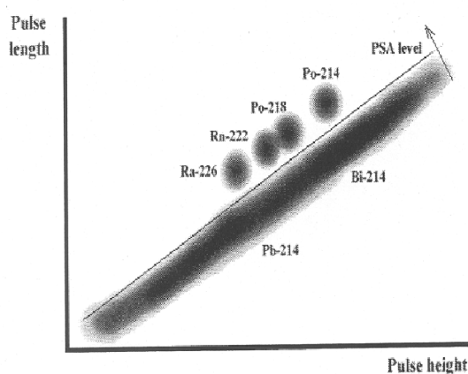
Fig. 9 3-D spectrum of Ra-226 vs. Pulse amplitude and Pulse length
