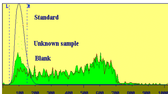
Fig. 10 Beta spectrum of tritium in rain
