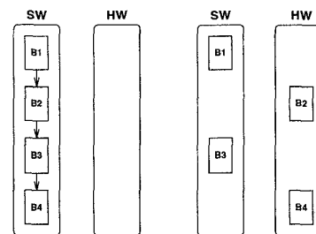
Figure 3: Partitioning model with instantaneous communication.
