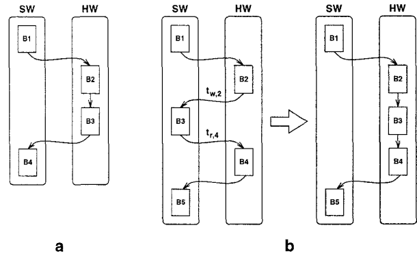
Figure 5: Partitioning model with adjacent block communication.
