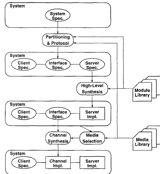
Figure 1: The communication synthesis flow for point-to-point communication.
