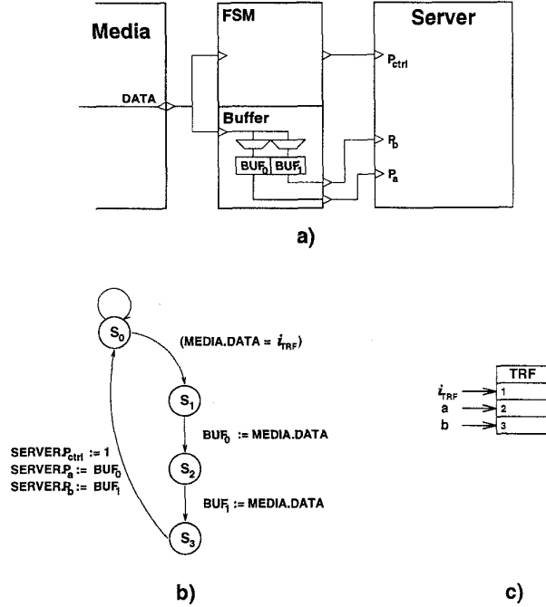
Figure 5: Channel hardware: a) overview, b) control unit FSM, c) client-end PFG.
