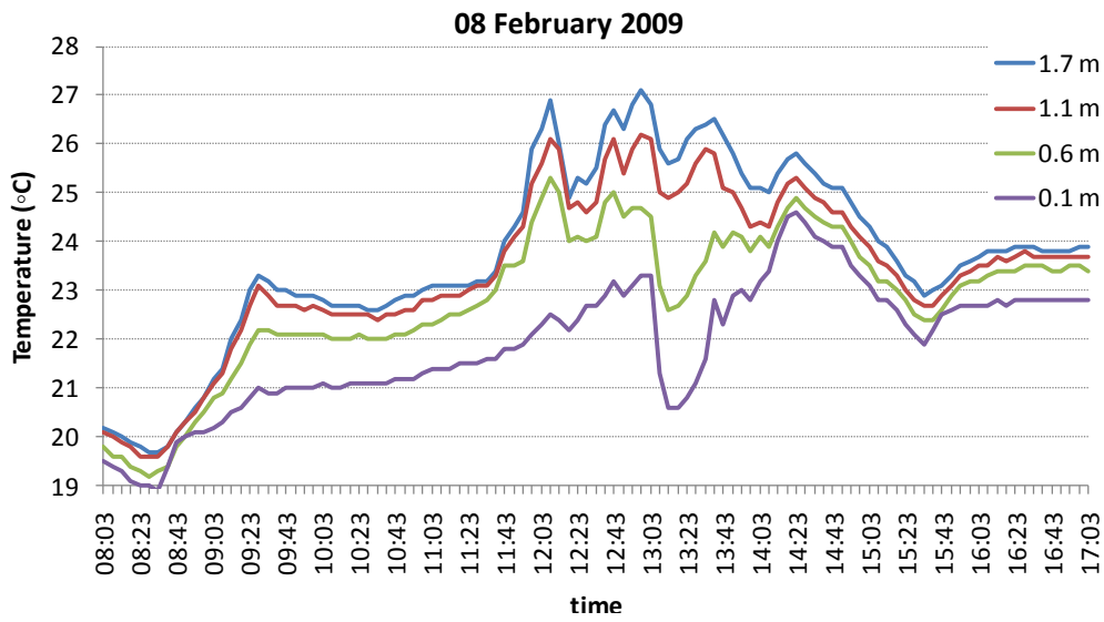
Figure 13. Vertical temperature distribution at 1 m's distance from the window (PRBS1).
