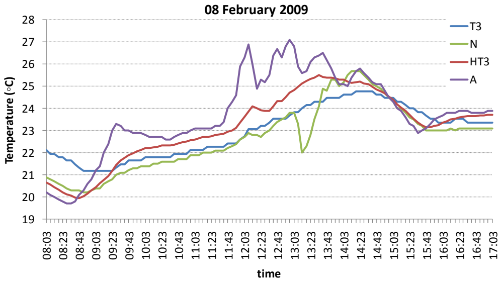
Figure 11. Temperatures measured by the heating control sensor, T3 , the sensor located on the wall at the same place, N , the HOBO, HT3 , and the occupied zone, A , during one day of working hours (PRBS1).
