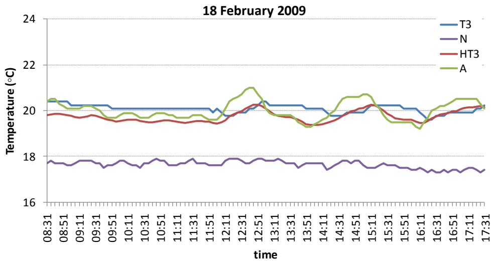
Figure 29. Temperatures measured by the heating control sensor, T3 , the sensor located at the same place on the wall, N , the HOBO, HT3 , and the occupied zone, A , during the working hours of one day (THERM1).
