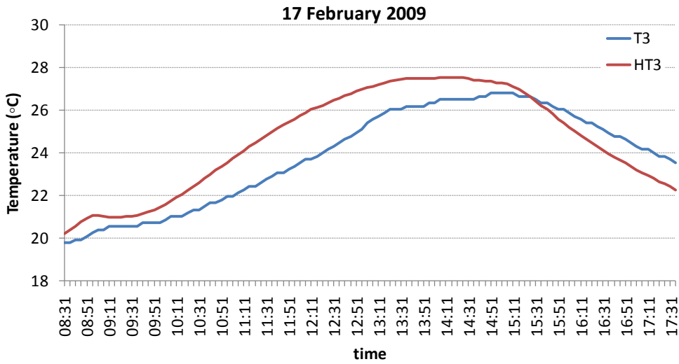
Figure 30. Detailed comparison of the temperatures measured by the heating control sensor, T3 , and HOBO, HT3 .
