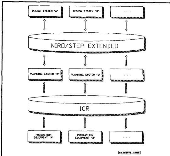
Figure 2.1. Conceptual schema for a CIME system architecture using the neutral interface concept [9].
