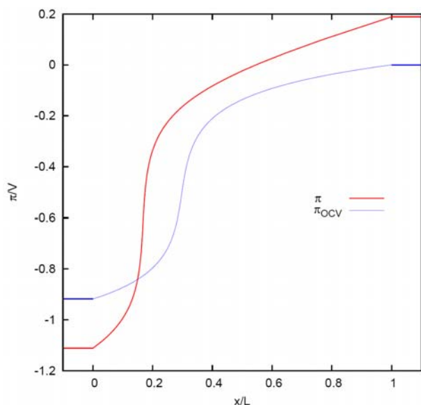
Figure 1: Electromotive potential, \pi , as function of relative distance from the interface between the negative electrode and the electrolyte in a cell operating in SOEC mode at the thermo-neutral cell voltage of 1.3 V compared to open circuit conditions at 1000 °C. x/L = 1 is the interface to the oxygen electrode. The electrolyte thickness was set to 200 \mu\text{m} , which gave an oxide ion current density of -2.1 \text{ A cm}^{-2} . The electron leak current density is \sim 10^{-4} \text{ A cm}^{-2} under the SOEC operation condition.
