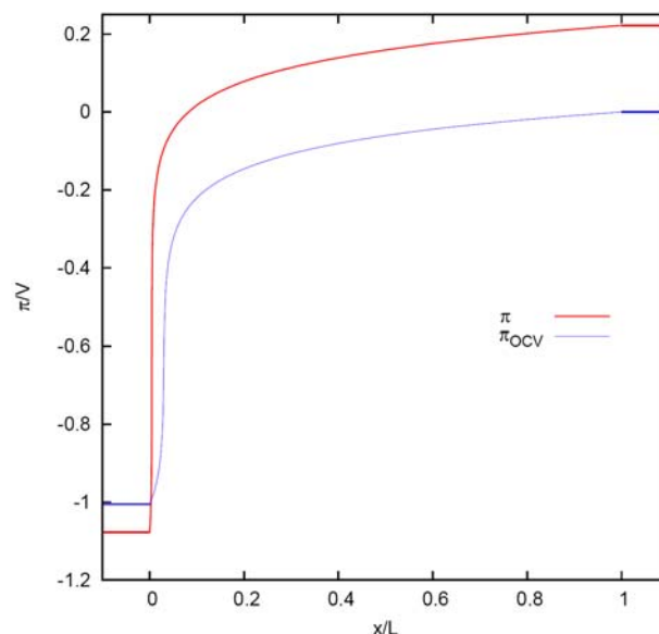
Figure 2: Electromotive potential, \pi , plotted like in Fig. 1 for 700 °C. The electrolyte thickness was set to 20 \mu\text{m} , which gave an oxide ion current density of -0.12 \text{ A cm}^{-2} . The electron leak current density is \sim 4 \cdot 10^{-6} \text{ A cm}^{-2} under the SOEC operation at 1.3 V.
