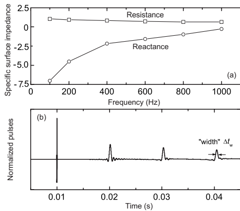
FIG. 1. (a) Specific surface impedance; (b) a series of a direct reflection and broadened reflected pulses up to the third reflection order (even spacing is assumed, and the magnitude is manipulated for clarity).
