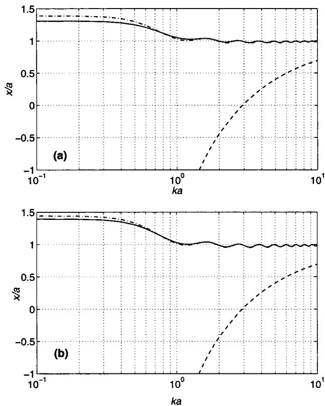
FIG. 3. The acoustic center of a point source on a rigid sphere of radius a seen from a distance of (a) five radii and (b) 10 radii. - \bullet - , First amplitude-based method [Eq. (18)]; - , second amplitude-based method [Eq. (19)]; - \cdot - , phase delay method [Eq. (21)].
