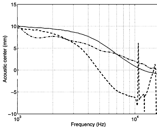
FIG. 4. Acoustic centers of microphones of type LS1 determined from the rate of change of the modulus of the transfer function ( - \bullet - ), and determined from the free-field phase response using the phase delay ( - ) and using the group delay ( - - ). The free-field phase response has been corrected for the phase of the pressure sensitivity.
