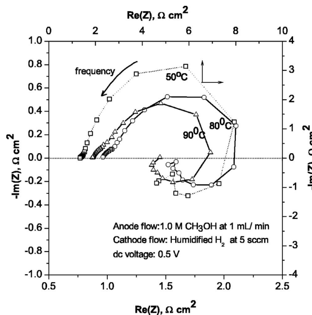
Figure 11. Nyquist plots showing the effect of temperature on methanol oxidation kinetics at the DMFC anode as determined by impedance spectroscopy at a dc voltage of 0.5 \text{ V} vs DHE. Anode: \sim 1.5 \text{ mg/cm}^2 Pt1Ru1. Cathode: \sim 2 \text{ mg/cm}^2 20% Pt/Vulcan carbon (E-TEK).
