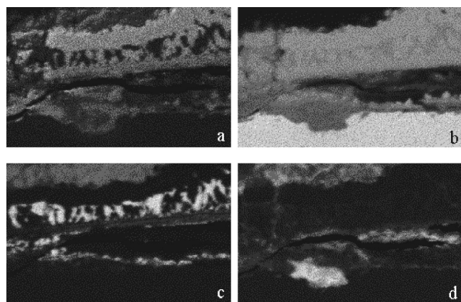
Figure 12. SEM element mapping of oxygen, iron, sulfur, and chlorine corresponding to Fig. 11: (a) oxygen, (b) iron, (c) sulfur, and (d) chlorine.
