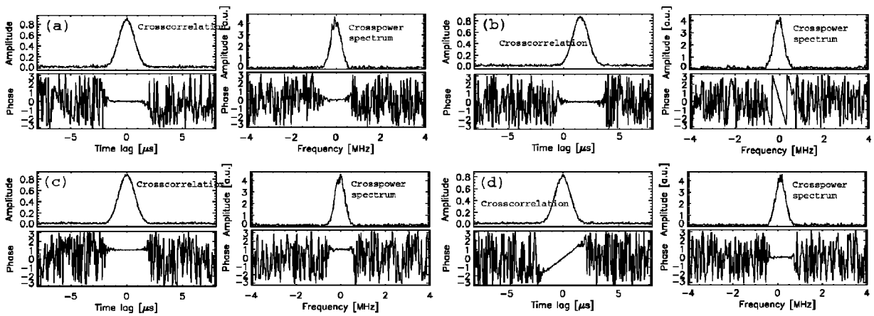
FIG. 7. Normalized correlation function and crosspower spectra of simulated signals. (a) \Delta_t=0, \Delta_\phi=0, v_\phi=0 , (b) \Delta_t=1.5 \mu s, \Delta_\phi=0, v_\phi=0 , (c) \Delta_t=0, \Delta_\phi=1, v_\phi=0 , (d) \Delta_t=0, \Delta_\phi=0, v_\phi=10^6 s^{-1} . See text for more explanation.
