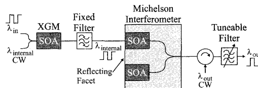
Fig. 1: Dual-stage wavelength converter
