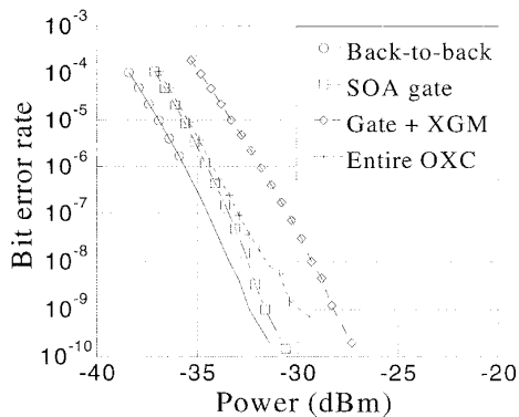
Fig. 4: Bit error rates measured through the OXC
