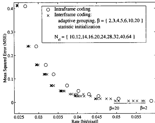
Fig. 4. Rate-distortion curve of Lloyd+PWC on the sequence "weather". Lossless coding is performed at 0.080 bpp in intra mode, 0.060 in inter mode.
