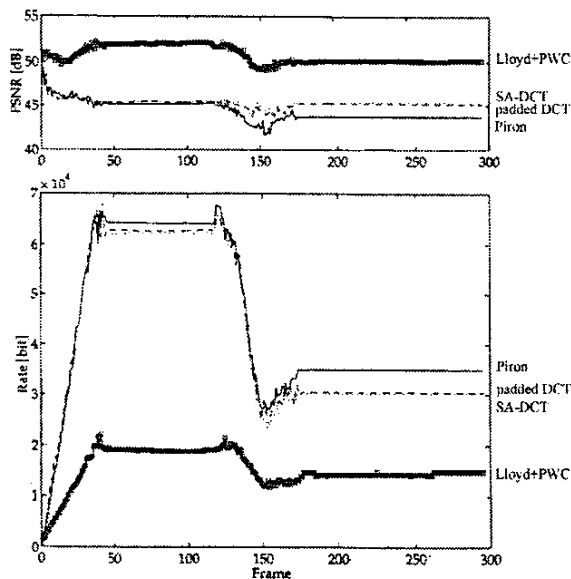
Fig. 5. Sequence "logo" (352 × 288 pixels): rate-distortion performances.
