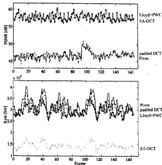
Fig. 6. Sequence "rain" (352 × 288 pixels): rate-distortion performances.
