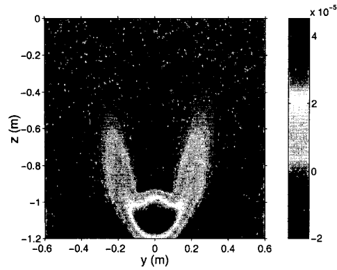
Figure 2: The image of \Delta\epsilon(y, z)/\epsilon_0 . The antennas are modeled as Hertzian dipoles.
