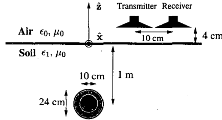
Figure 1: The fixed-offset GPR configuration involving a two-layer circular pipe. The antennas are resistively loaded \hat{x} -directed dipoles.
