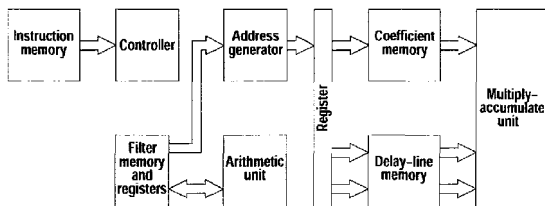
Figure 4. Block diagram of the FIR mini-core.
