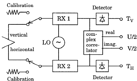
Figure 1: Basic correlation radiometer.
