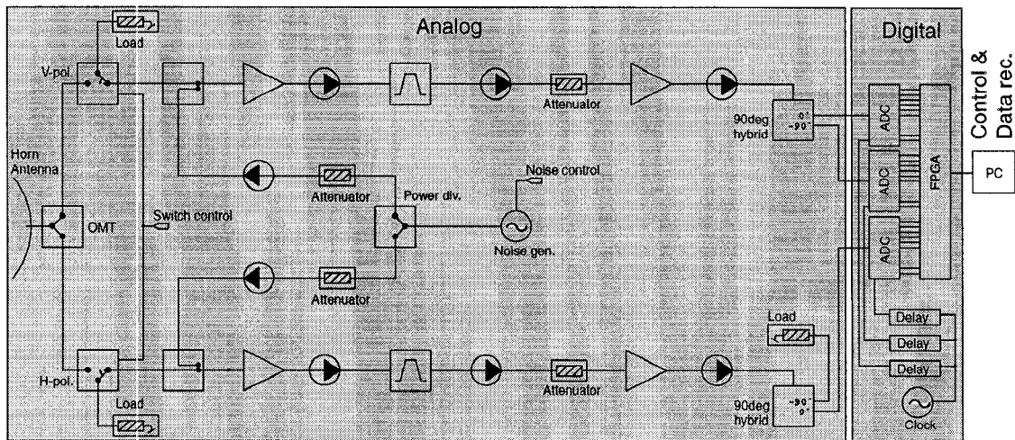
Figure 2: Subharmonic sampling correlation radiometer.
