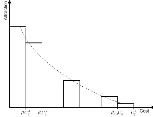
Figure 2: Attraction function approximated by a step-function.
