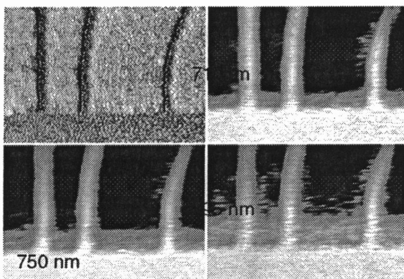
Figure 2: Waveguiding of surface plasmon polaritons at different excitation wavelengths. The top left figure illustrates the topography of the sample surface. Each image represents the same 32\ \mu\text{m} \times 22\ \mu\text{m} area. The plasmon polaritons propagate from bottom to top in the figures.
