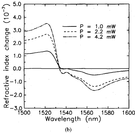
Fig. 3. Measured (a) and calculated (b) refractive index change as function of signal wavelength for fiber A ( \text{Er}^{3+} -doping concentration of 0.7 \times 10^{19} \text{ cm}^{-3} ) at an absorbed pump power of 1.0 mW (circular symbols and solid curves), 2.2 mW (square symbols and dashed curves) and 4.2 mW (triangular symbols and dashdotted curves). The wavelength of the pump power is 980 nm. The threshold pump power P_{th} has been set equal to 0.8 mW and the offsets for the calculated solid, dashed, and dashdotted curves in (a) have been set equal to 0.4 \times 10^{-7} , 0.8 \times 10^{-7} and 1.1 \times 10^{-7} , respectively (see text).
