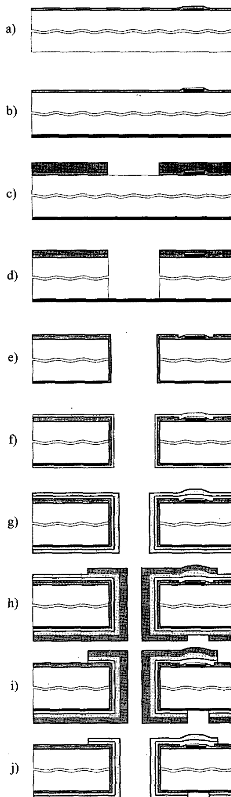
Figure 2: Simplified process sequence for post processing of through-wafer vias in CMOS wafers.
