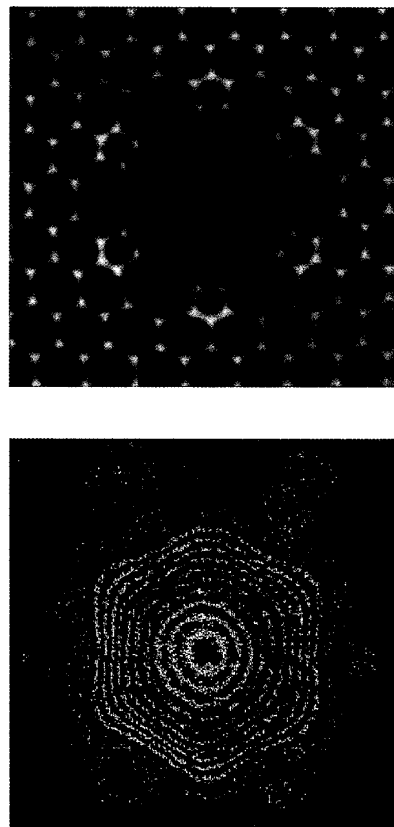
Fig. 7. Microscope picture of a single-mode hollow-core PBG fiber (top), and a near-field image of the guided mode profile (bottom).
