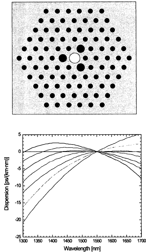
Fig. 2. The generic structure of a Ge/F-doped PCF with flattened dispersion around 1500 nm wavelength (top). Darker regions have lower refractive index. In the bottom panel, some simulated dispersion curves are shown.
