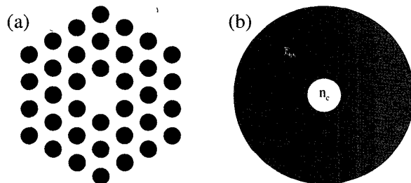
Fig. 1. (a) The most common PCF design at present. Dark areas are airholes while white areas are silica. (b) Effective index model of the design in (a).
