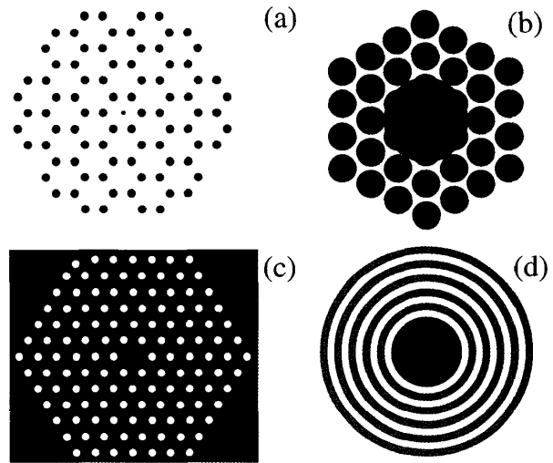
Fig. 6. Schematic pictures of various photonic bandgap (PBG) fiber designs. Lighter color indicates higher refractive index. (a) Honeycomb PBG fiber with central hole defect. (b) Airguiding PBG fiber. (c) PBG fiber with a triangular array of high-index rods, formed e.g. by liquid-filling of the holes in a standard index-guiding PCF. (d) Omniguide PBG fiber.
