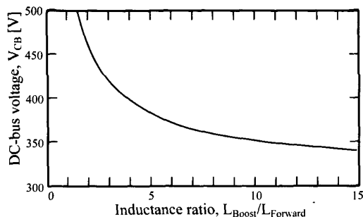
Figure 3. DC-Bus Voltage as a Function of Boost-Forward Inductor Ratio. The Plot Applies for V_{AC} = 230V , V_{OUT} = 70V and n_{12} = 1.5 .
