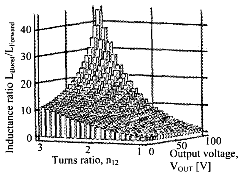
Figure 4. Boost-Forward Inductance Ratio as a Function of the Turns Ratio and Output Voltage. The Plot Applies for V_{AC} = 230V and DC-Bus Voltage V_{CB} = 400V .
