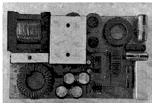
Figure 12. The Experimental Two-Switch Boost-forward Single-Stage PFC Power Supply.
