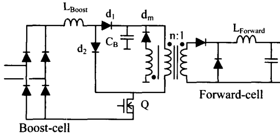
Figure 2. Single-Stage Power Supply Using Boost-Forward Topology.
