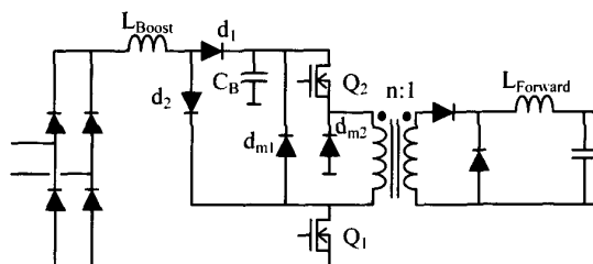
Figure 5. Single-Stage Power Supply Using the Two-Switch Boost-Forward Topology.
