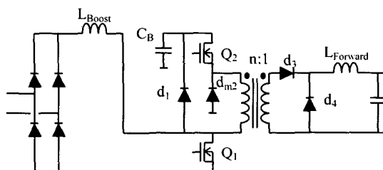
Figure 6. Simplified Version of the Single-Stage Power Supply Using the Two-Switch Boost-Forward Topology.
