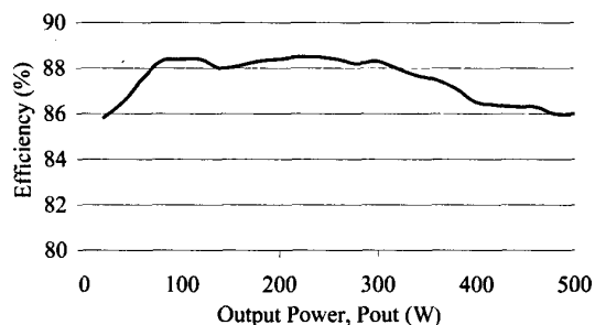
Figure 9. Measured Efficiency as a Function of Output Power.
