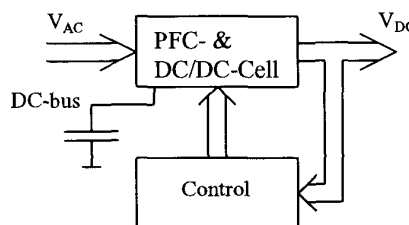
Figure 1b. Single-Stage Converter. DC/DC Control Circuit
