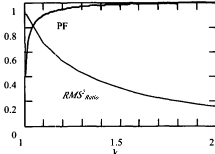
Figure 8. RMS^2 Ratio and PF as a Function of k
