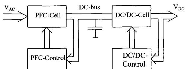
Figure 1a. Two-Stage Converter. Separate Control of PFC and DC/DC Conversion.
