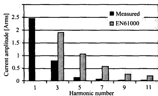
Figure 11. Measured Current Harmonics at 564W Input Power and the Limits Given by EN61000-3-2 Class D.
