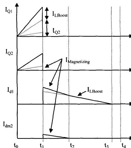
Figure 7. Primary Side Current Waveforms for the DCM Two-Switch Boost-Forward Topology of Figure 6.
