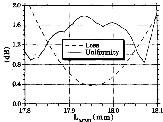
Fig. 7. Loss and uniformity versus the length of the multimode section of the 1-by-64 MMI power splitter with the width fixed at 1.105 mm.
