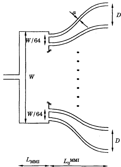
Fig. 1. Geometry of 1-by-64 MMI power splitter. The cladding refractive index is n_2 and the core refractive index is n_1 .
